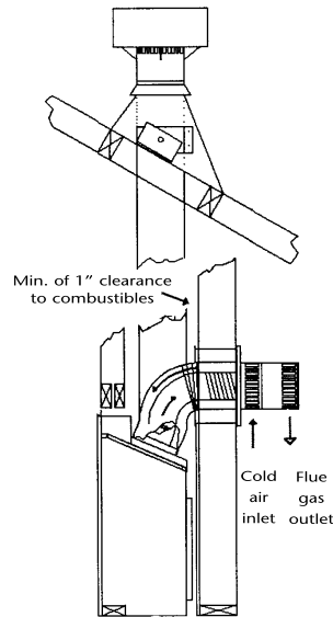
Unit illustrated is a ZDV3318N Zero Clearance Direct Vent Fireplace – Natural Gas, with LOGC50 Log Set, Z6GCR Grill Kit – Chrome.
